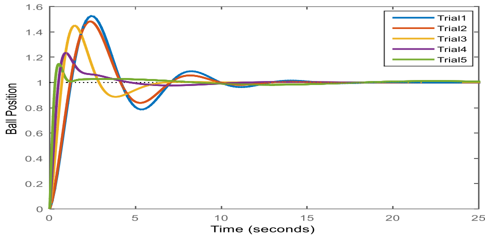
Figure 8: The step response of the system with various trials
