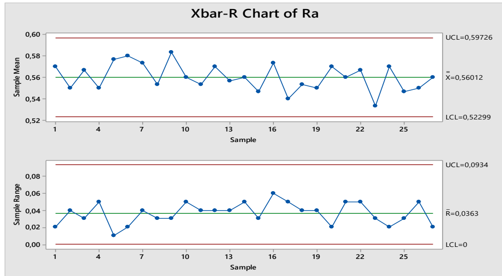
Figure 1: X-bar & R control chart for Roughness R_a
