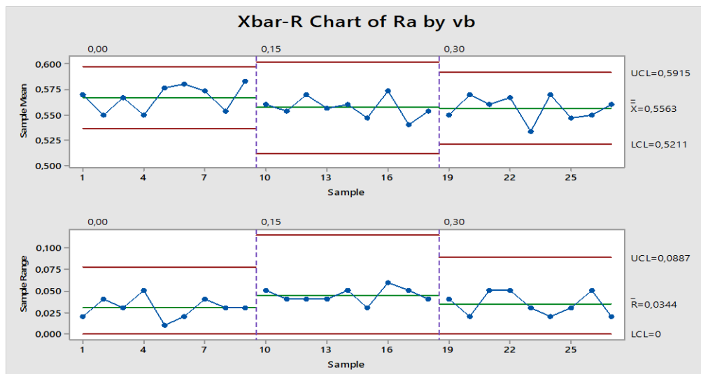
Figure 2: Roughness R_a controlgraph regarding tool wear ( v_b )
