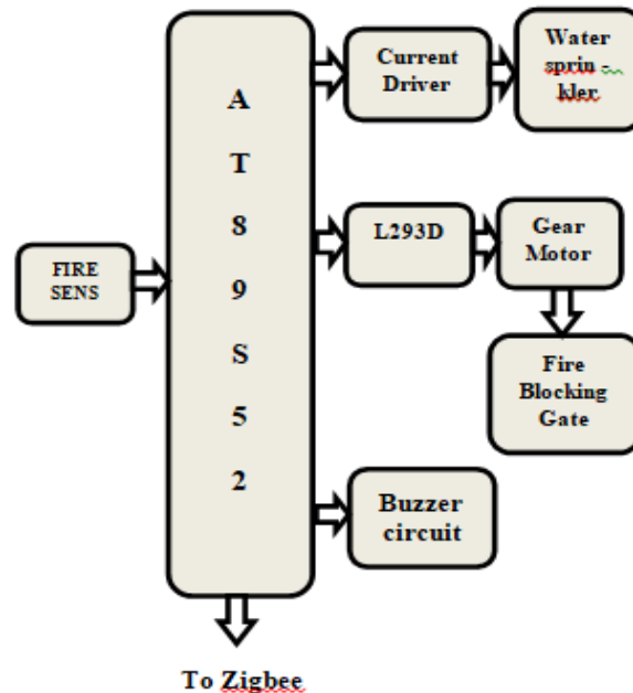
Figure 2: Fire controlling circuit
