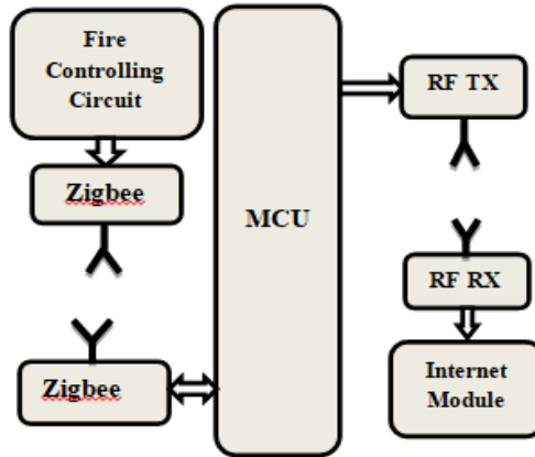
Figure 1: Complete system design
