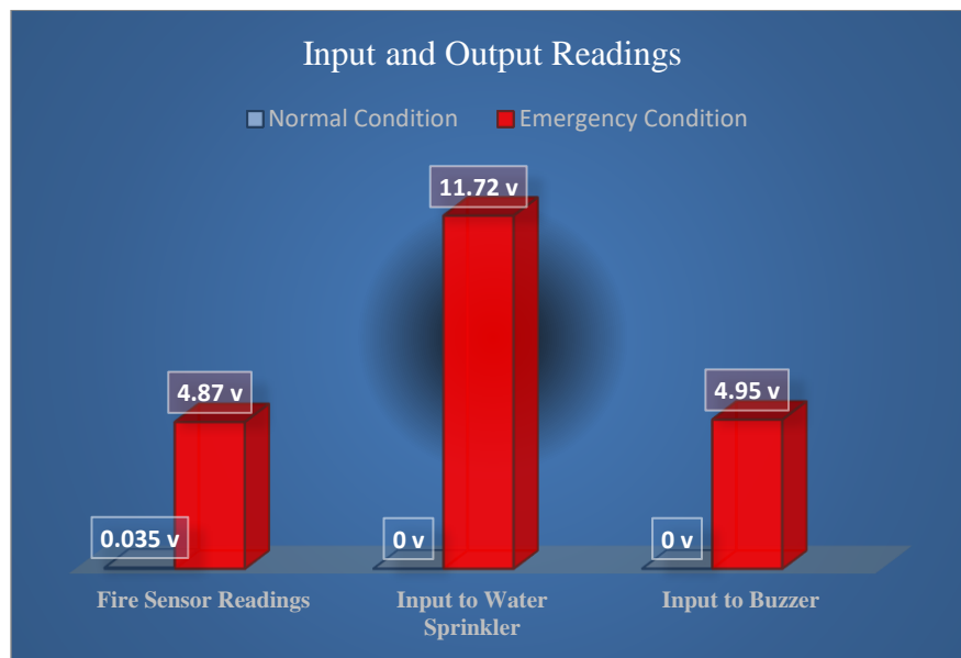
Figure 3: Sensor and Actuator voltages
