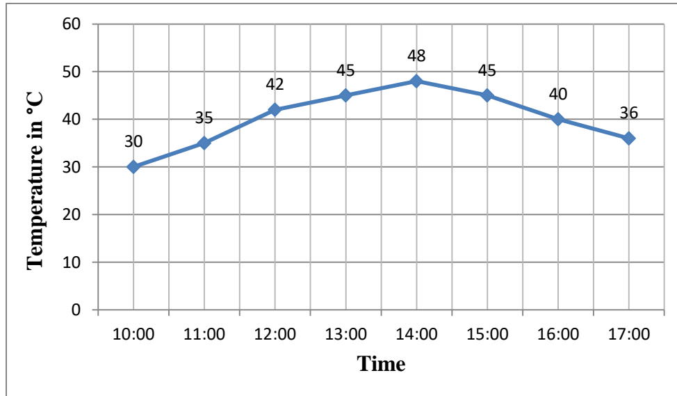
Figure 6: Time and temperature with water flow rate 15 litres/ Minutes
