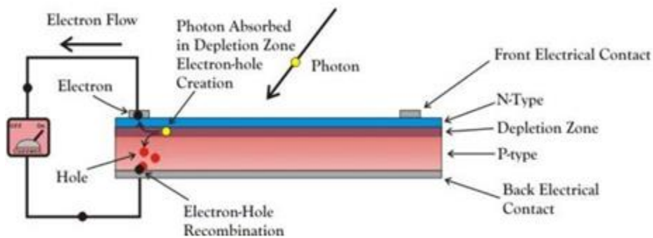
Figure 4: Solar Cell
