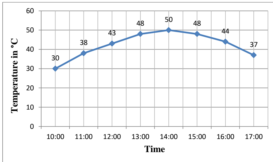
Figure.7. Time and temperature with water flow rate 16 litres/ Minutes
