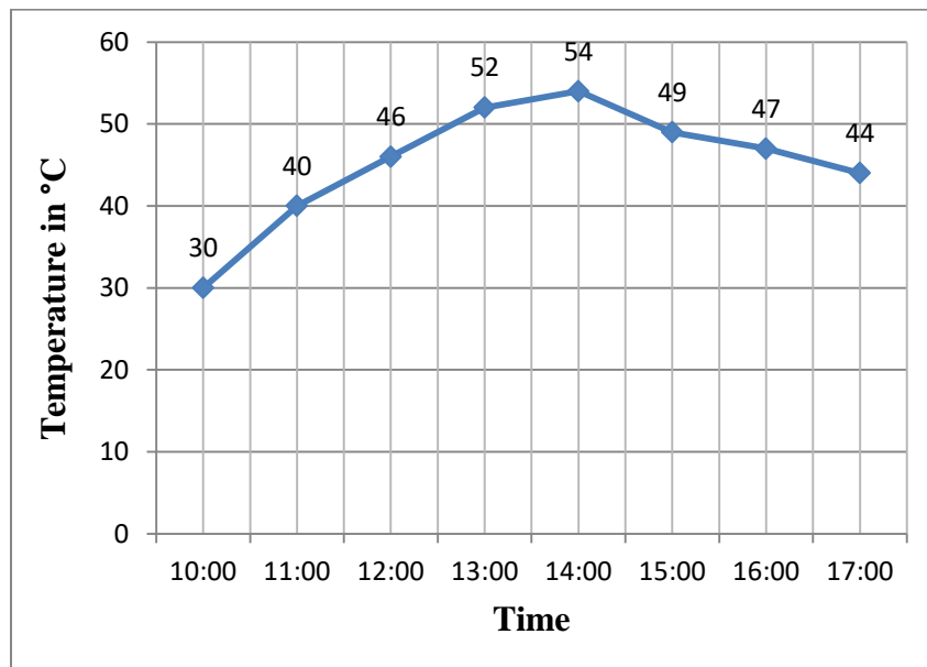
Figure 10: Time and temperature with water flow rate 19 litres/ Minutes
