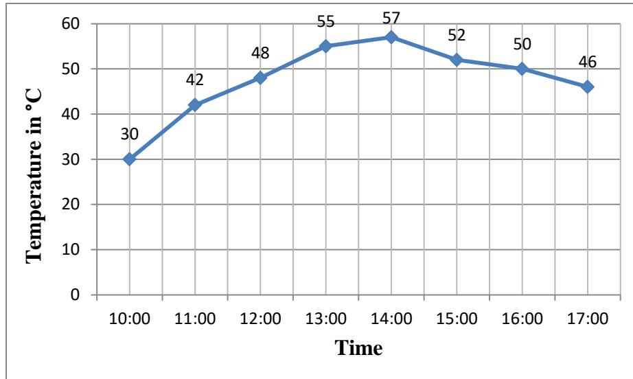
Figure 9: Time and temperature with water flow rate 18 litres/ Minutes
