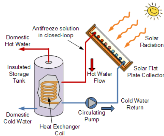
Figure 3: Indirect Hot Water System
