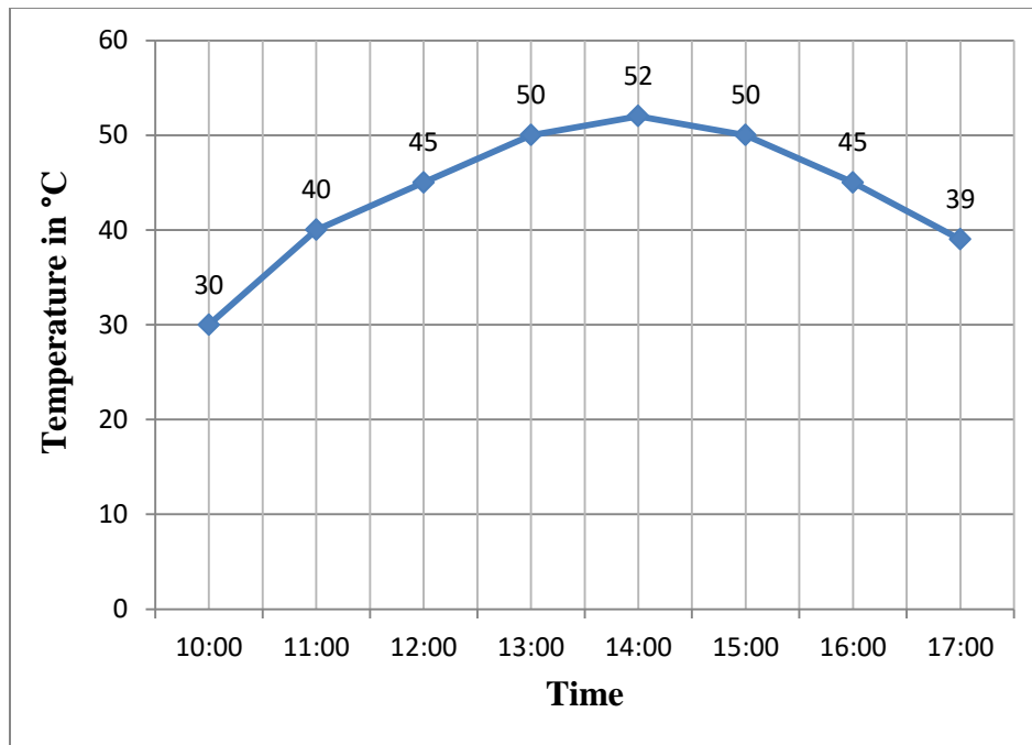
Figure 8: Time and temperature with water flow rate 17 litres/ Minutes
