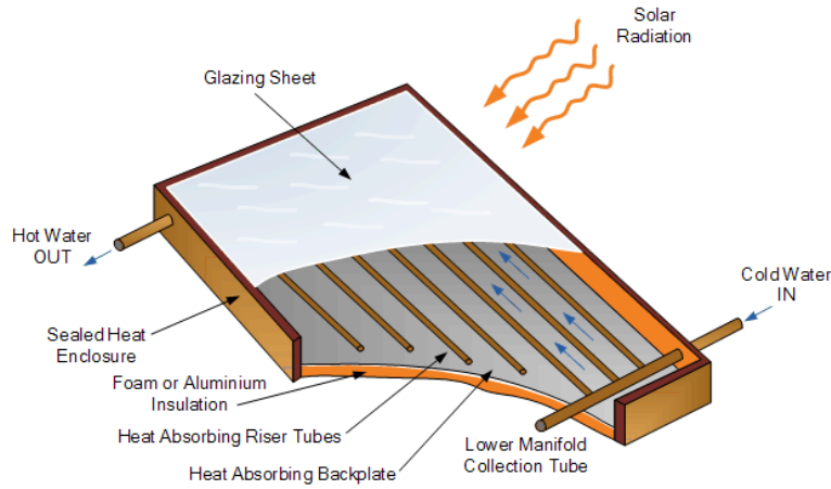
Figure 2: Flat Plate Collector
