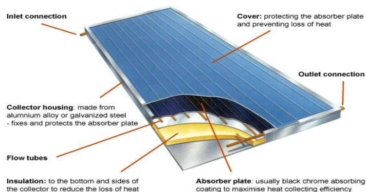
Figure 1: solar heating system
