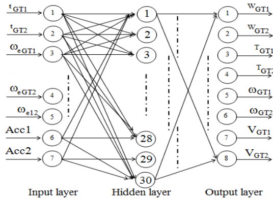
Figure 6: The structure of ANN to control observer
