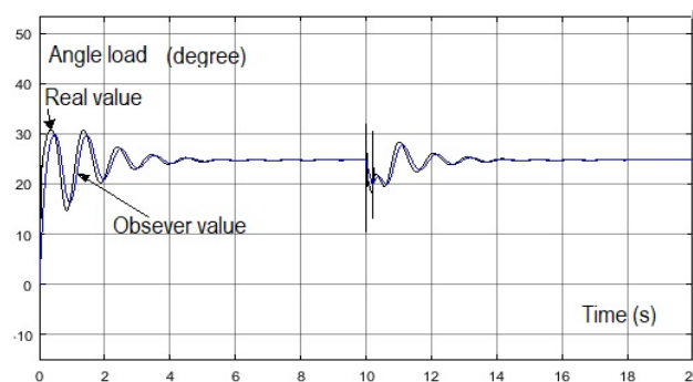
Figure 8: Result of observer for load angle
