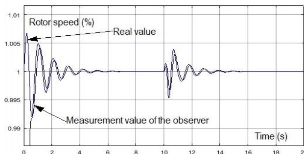
Figure 9: Result of the speed measurement
