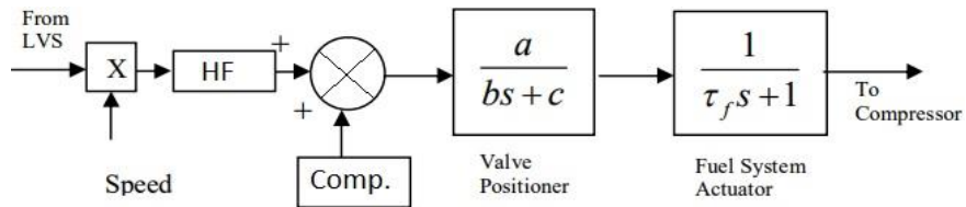
Figure 3: Modelling of the fuel valve structure
