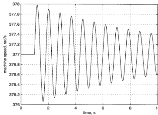
Figure 1: A local oscillation in the power system
