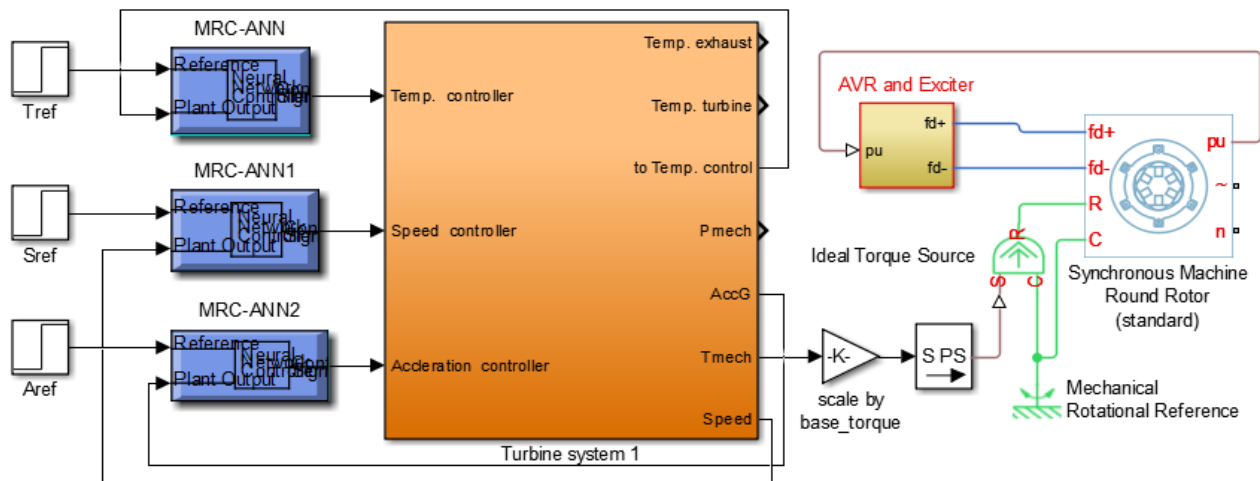
Figure 5: Model of turbine and generator
