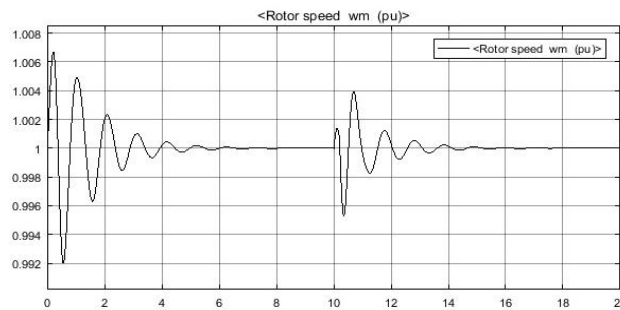
Figure 7: The change speed when change power load
