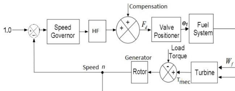
Figure 2: A basic model of gas turbine generator plant
