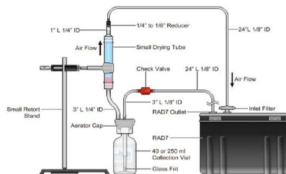
Figure 3: Schematic Diagram of RAD7 Detector with RAD H 2 O Accessories.
