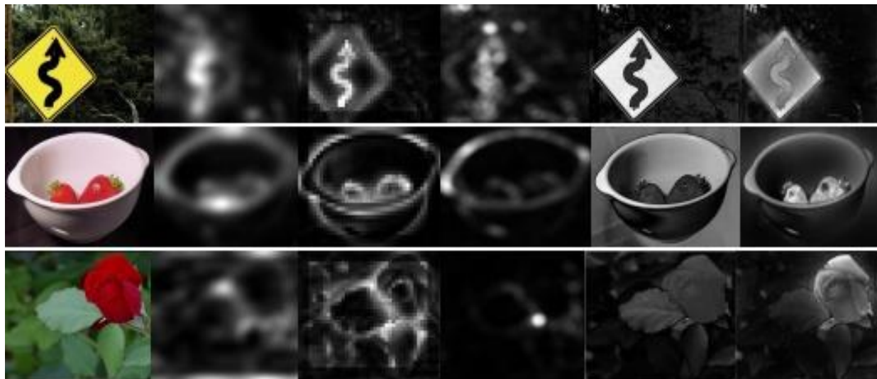
Figure 2: Sample color images, and saliency maps of IT [5], MZ [6], SR [7], FT [4], and proposed model
