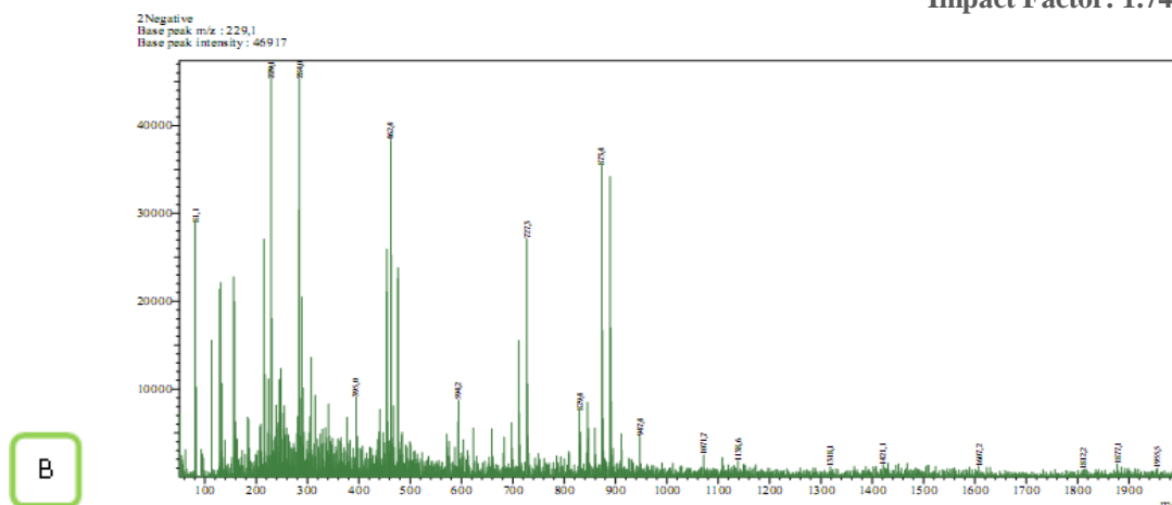
Figure 3: Chromatogram of the relative content of phenolic compounds in Zygophyllum album plant (A: ESI+ ;B :ESI-)
