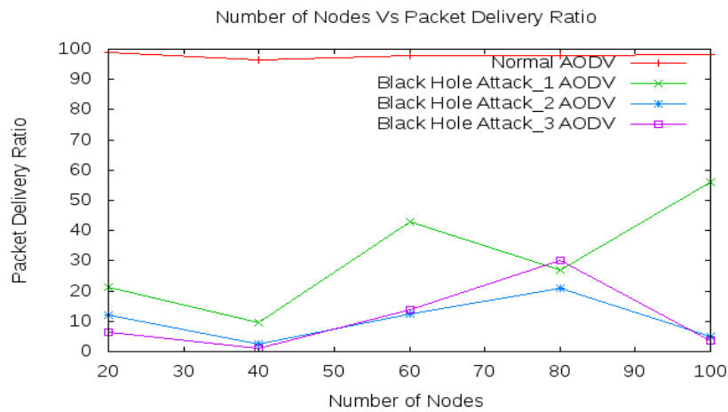
Figure 2: Packet delivery ratio of normal AODV and black hole attack AODV
