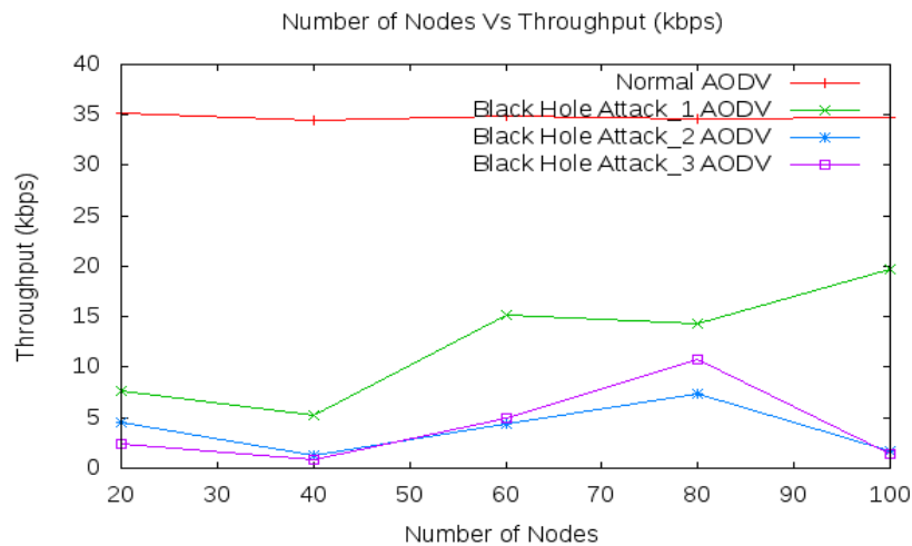
Figure 3: Throughput of normal AODV and black hole attack AODV
