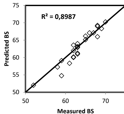
Figure 4: BS value comparison of experimental and ANN model data for tested samples
