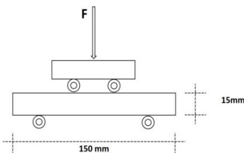
Figure 2: 4-point bending test scheme
