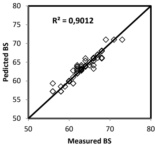
Figure 3: BS value comparison of experimental And ANN model data for trained samples
