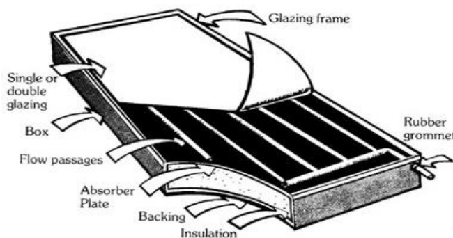
Figure1: Solar water heater
