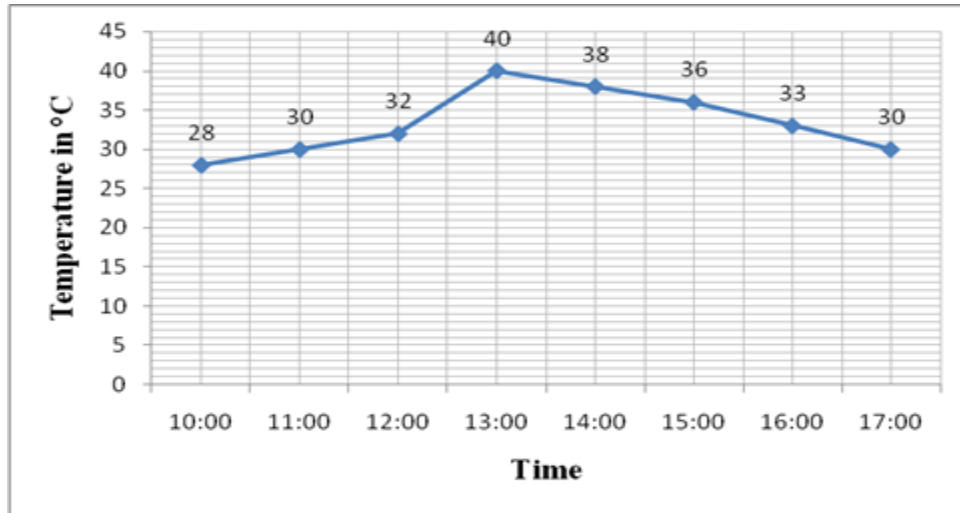
Figure 3: Time and temperature with water flow rate 6 liters/ Minutes
