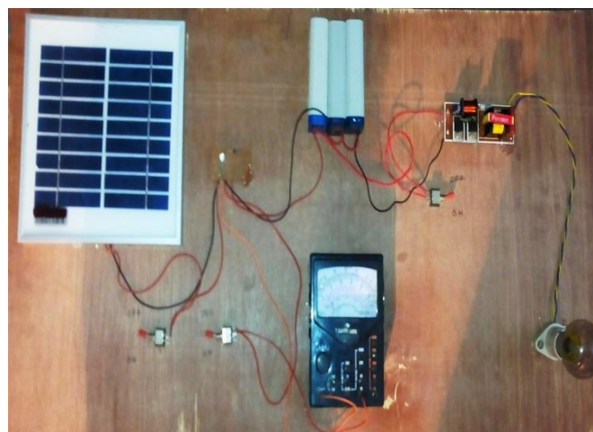
Figure 3: Experimental Setup
