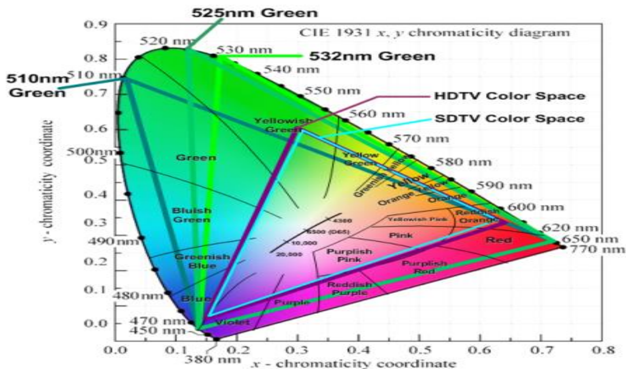
Figure 1: Chromaticity Diagram
