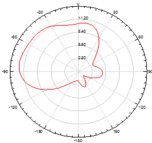
Figure 3: (c) Radiation pattern at 7.5 GHz
