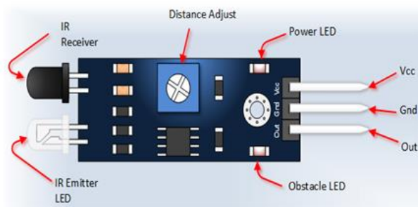
Figure 2: IR SENSOR [2]
